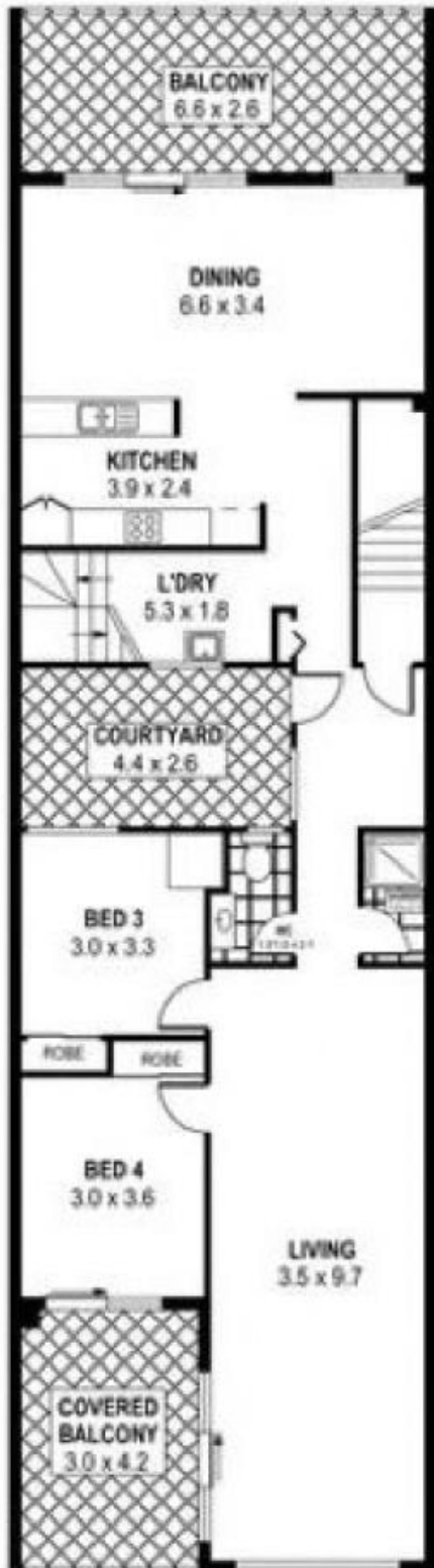
FIRST FLOOR
