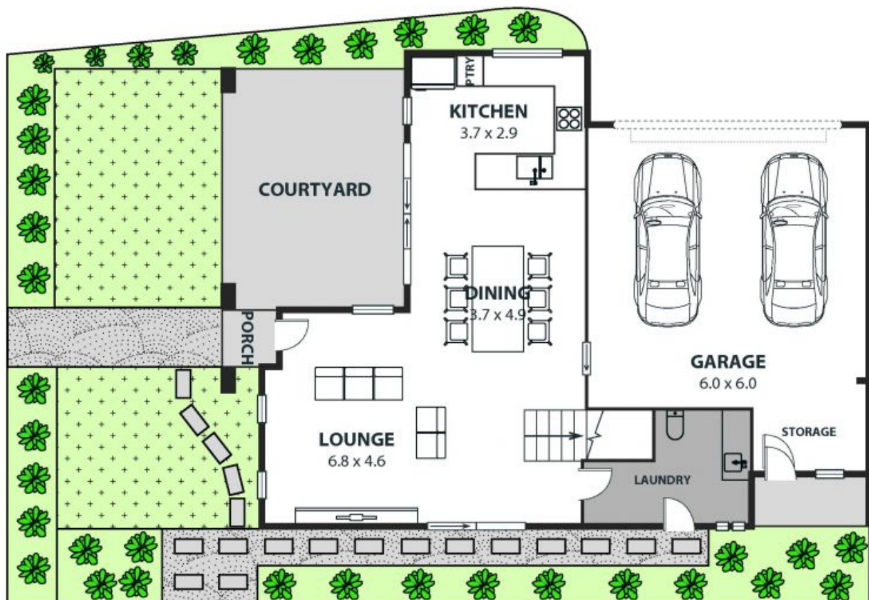
GROUND FLOOR
